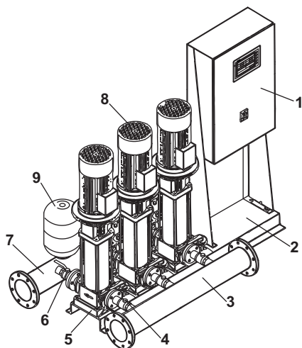
FIG. 4 SYSTEM COMPONENTS
